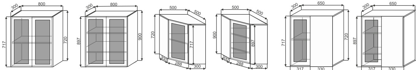
BC 800 800x720x300 BC(2) 800 800x900x300 ВУС 500X500 500x720x500 ВУС(2) 500X500 500x900x500 ВСУ 650 650x720x300 ВСУ(2) 650 650x900x300
