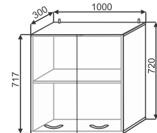
ШВ 1000 1000x720x300
