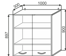
ШВ(2) 1000 1000x900x300
