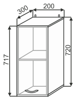
ШВ 200 200x720x300
