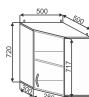
ШВУ 500X500 500x720x500
