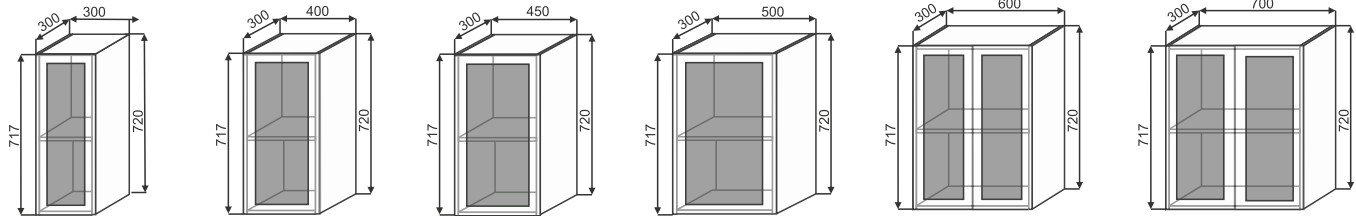
BC 300 300x720x300 BC 400 400x720x300 BC 450 450x720x300 BC 500 500x720x300 BC 600 600x720x300 BC 700 700x720x300
