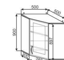
ШВУС(2) 500X500 500x900x500
