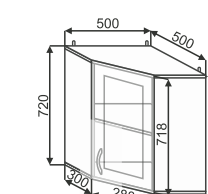
ШВУС 500X500 500x720x500
